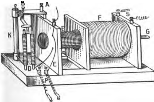
Induction coil.
